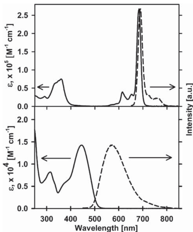
FIGURE 1. Steady-state absorption (solid line) and normalized fluorescence (dashed line) spectra of compounds 1 (top) and 3 (bottom).
