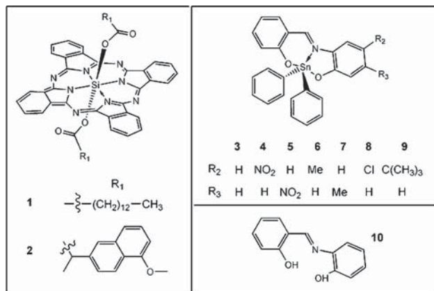
SCHEME 1. Molecular structures of the compounds of this study.
