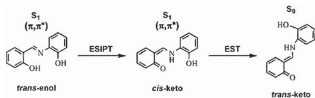
SCHEME 2. Resumed photoinduced pathway of the free Schiff base 10 showing the excited state intramolecular proton transfer (ESIPT) and excited state tautomerization (EST). Besides the tautomerization towards the trans-keto form, depletion of the cis-keto isomer is also due to other radiationless processes [13-15].
