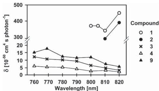
FIGURE 2. Two-photon absorption cross sections ( \delta ) of 1 and 2 in dichloromethane solution, and 3 , 4 , and 9 in ethanol solution. Standard deviations from three independent measurements are of approximately 15%.
